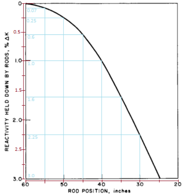
Figure 4.5: Control rod 1 calibration (Kirn et al., 1960).
